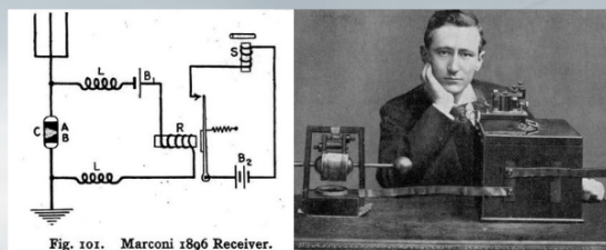
Fig. 101. Marconi 1896 Receiver.
